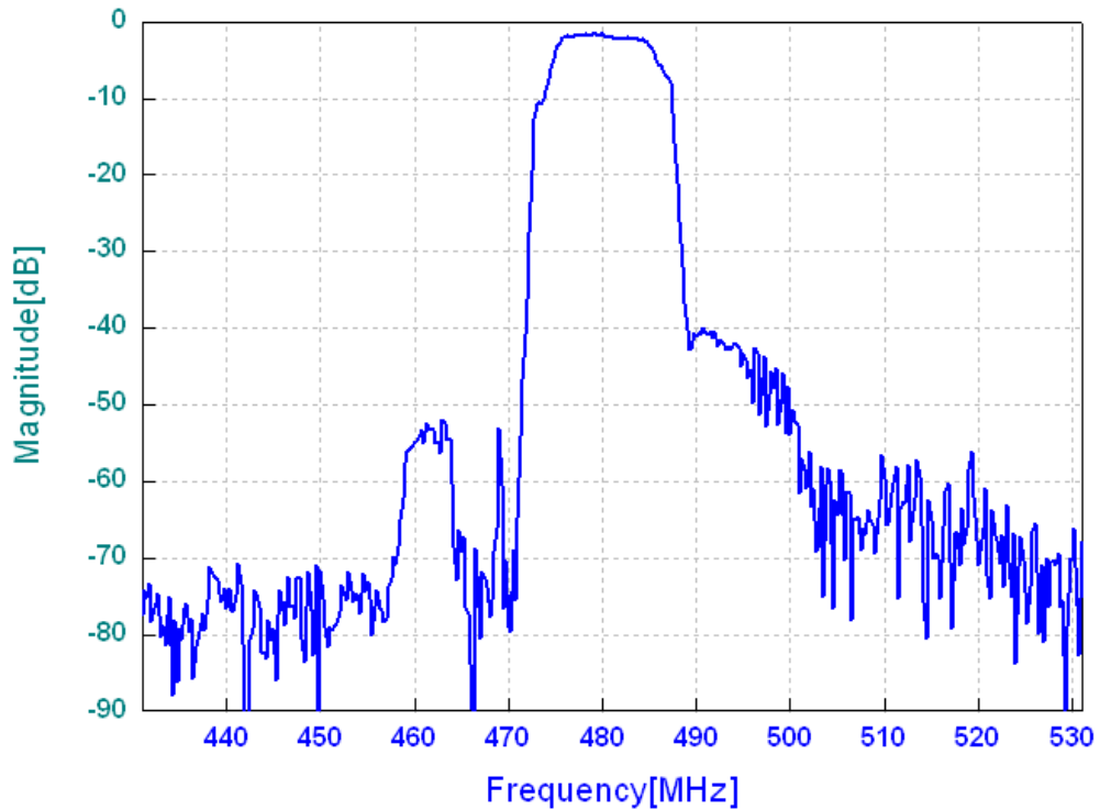
Frequency Response
